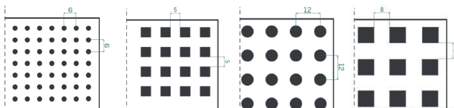
Perforado 5x5 23% perforado
